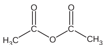
Ethanoic anhydride
